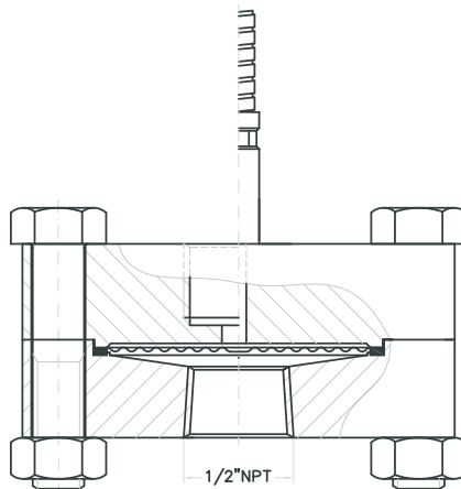
Threaded female process connection
