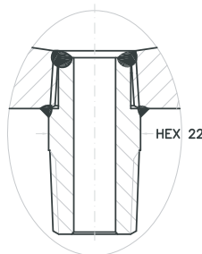
Threaded male process connection
