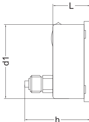
type D (Ø 63 mm, without blow-out back)
