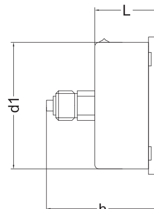
type D Ø 50 mm
