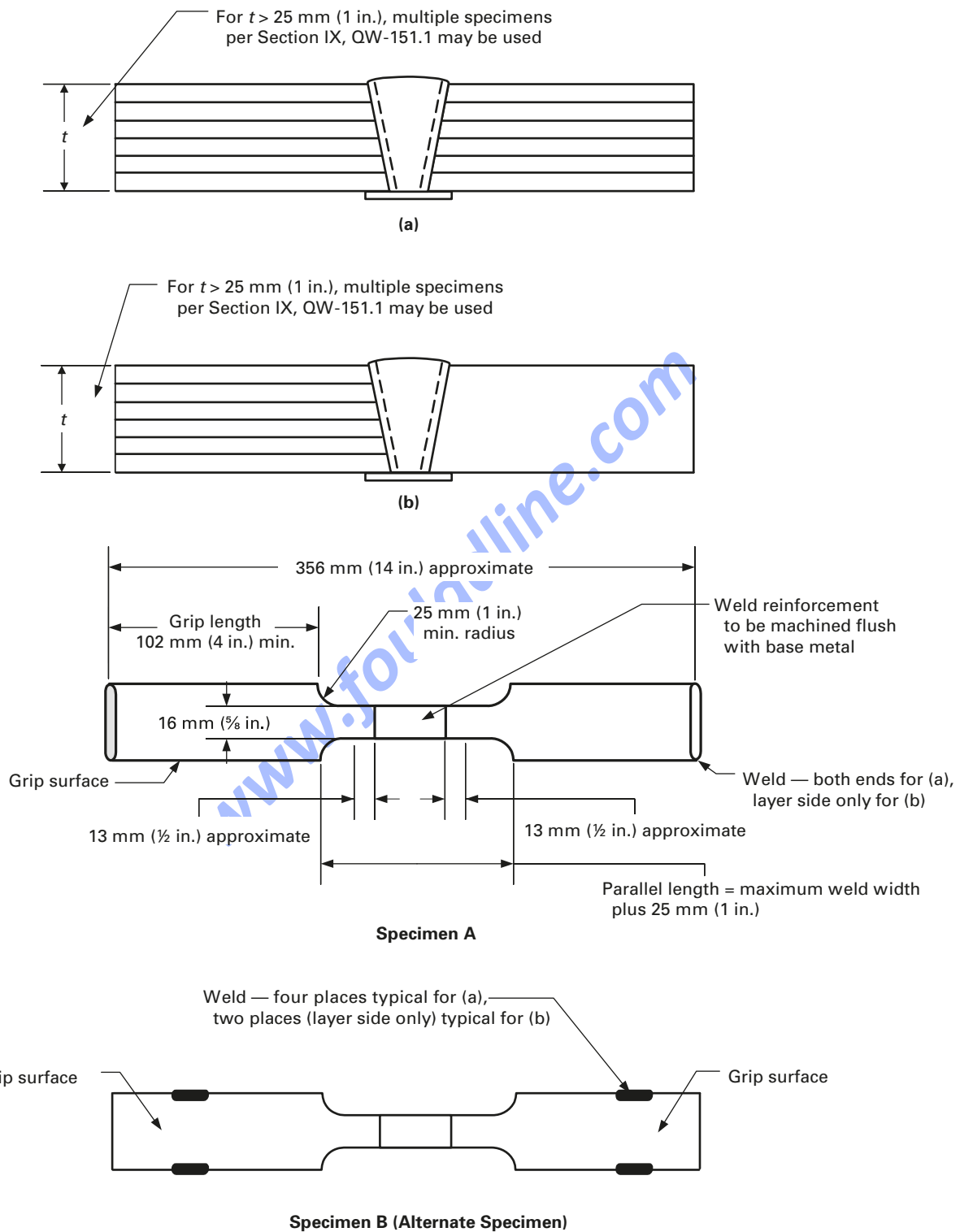
Figure 6.5 Tensile Specimens for Layered Vessel Construction
