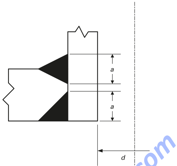
Figure 7.17 Dimensions a and d for a Partial Penetration Corner Weld
