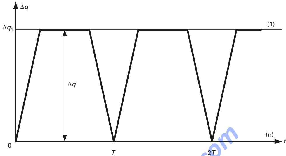
Figure 4.19.8 Cyclic Displacements
