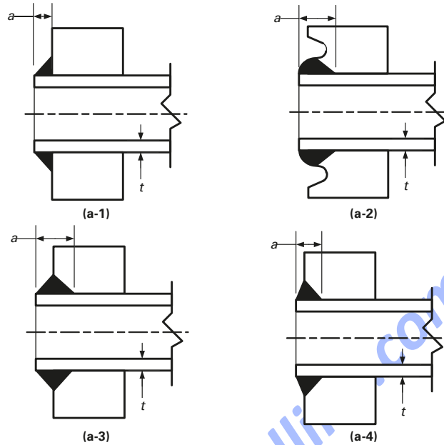
(a) Some Acceptable Weld Geometries Where a Is Greater Than or Equal to 1.4t
