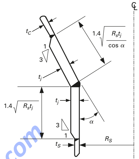
Figure 4.3.9 Reinforcement Requirements for Conical Transition Junction
