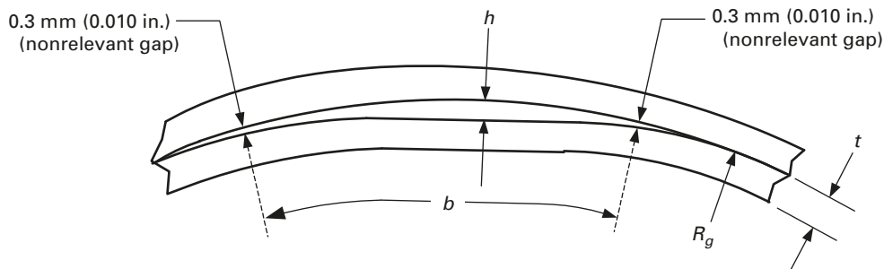
Figure 4.13.11 Gap Between Vessel Layers
