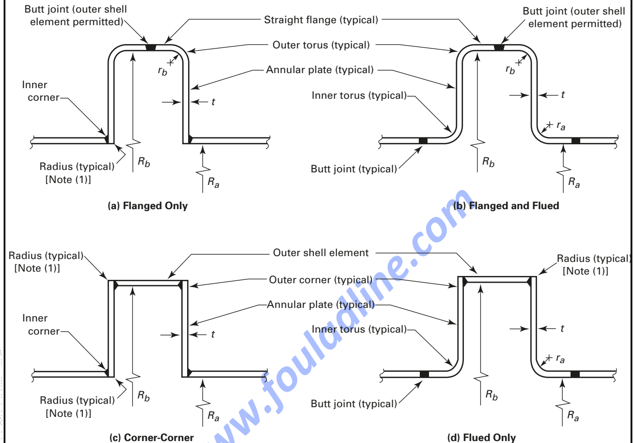
Figure 4.20.1 Typical Flexible Shell Element Expansion Joints
