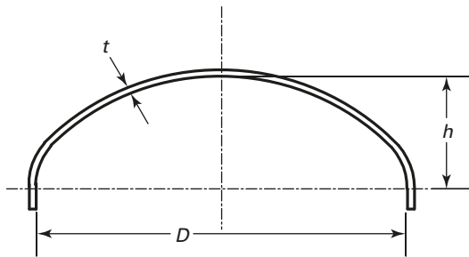
Figure 4.3.5 Ellipsoidal Head
