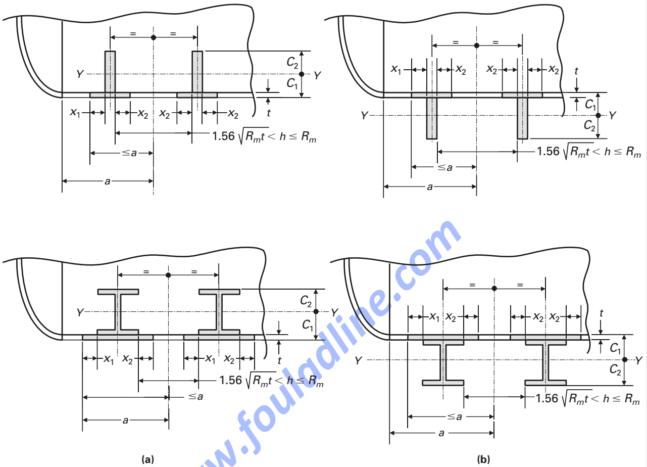
Figure 4.15.4 Cylindrical Shell With Stiffening Rings on Both Sides of the Saddle
