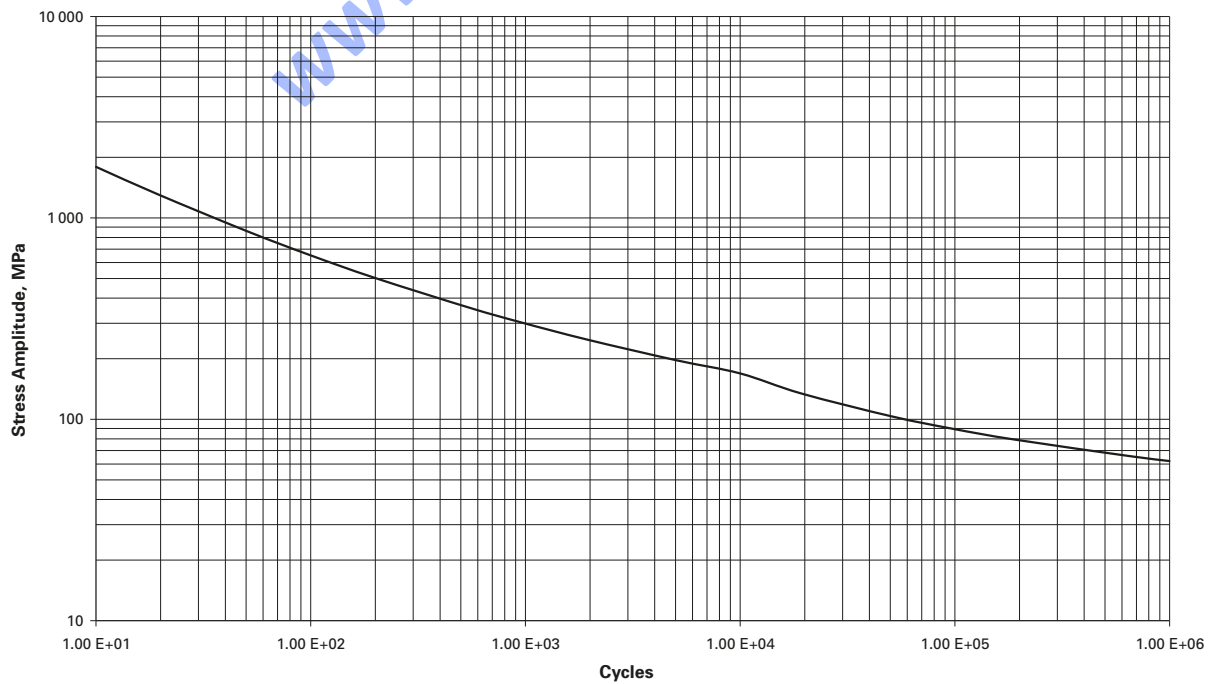
Figure 3-F.5M Fatigue Curve for Wrought 70–30 Copper–Nickel for Temperatures Not Exceeding 371°C — \sigma_{ys} = 207 MPa
