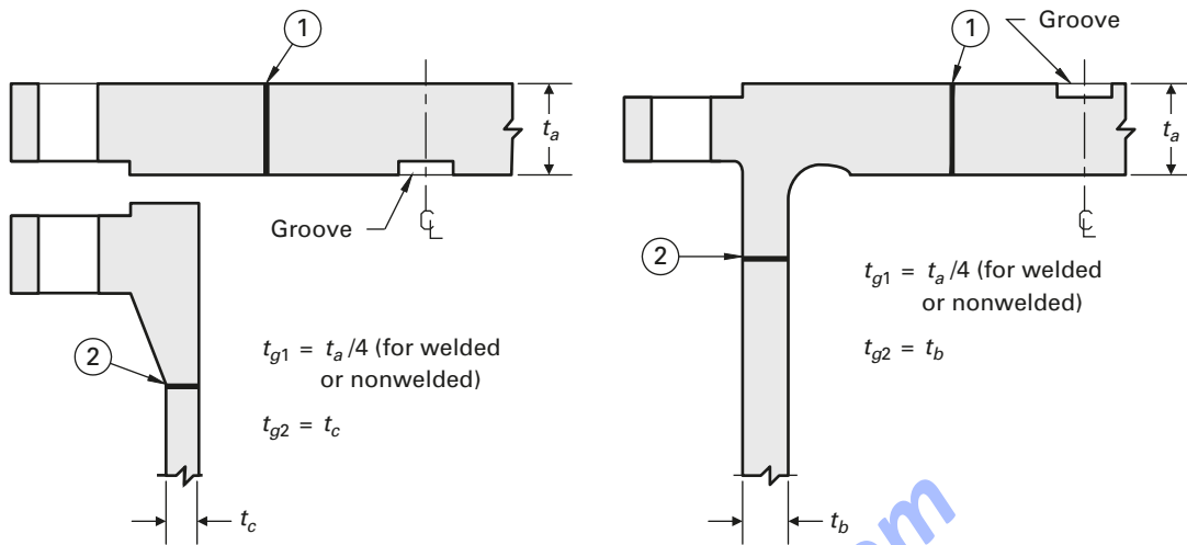
Figure 3.10 Typical Vessel Details Illustrating the Governing Thickness
