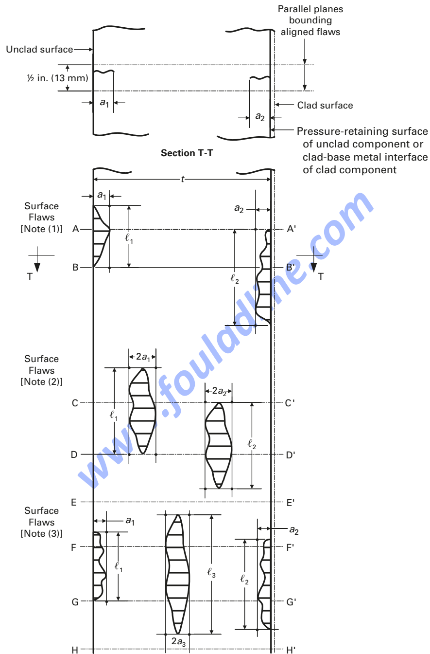
Figure 7.15 Multiple Aligned Planar Flaws
