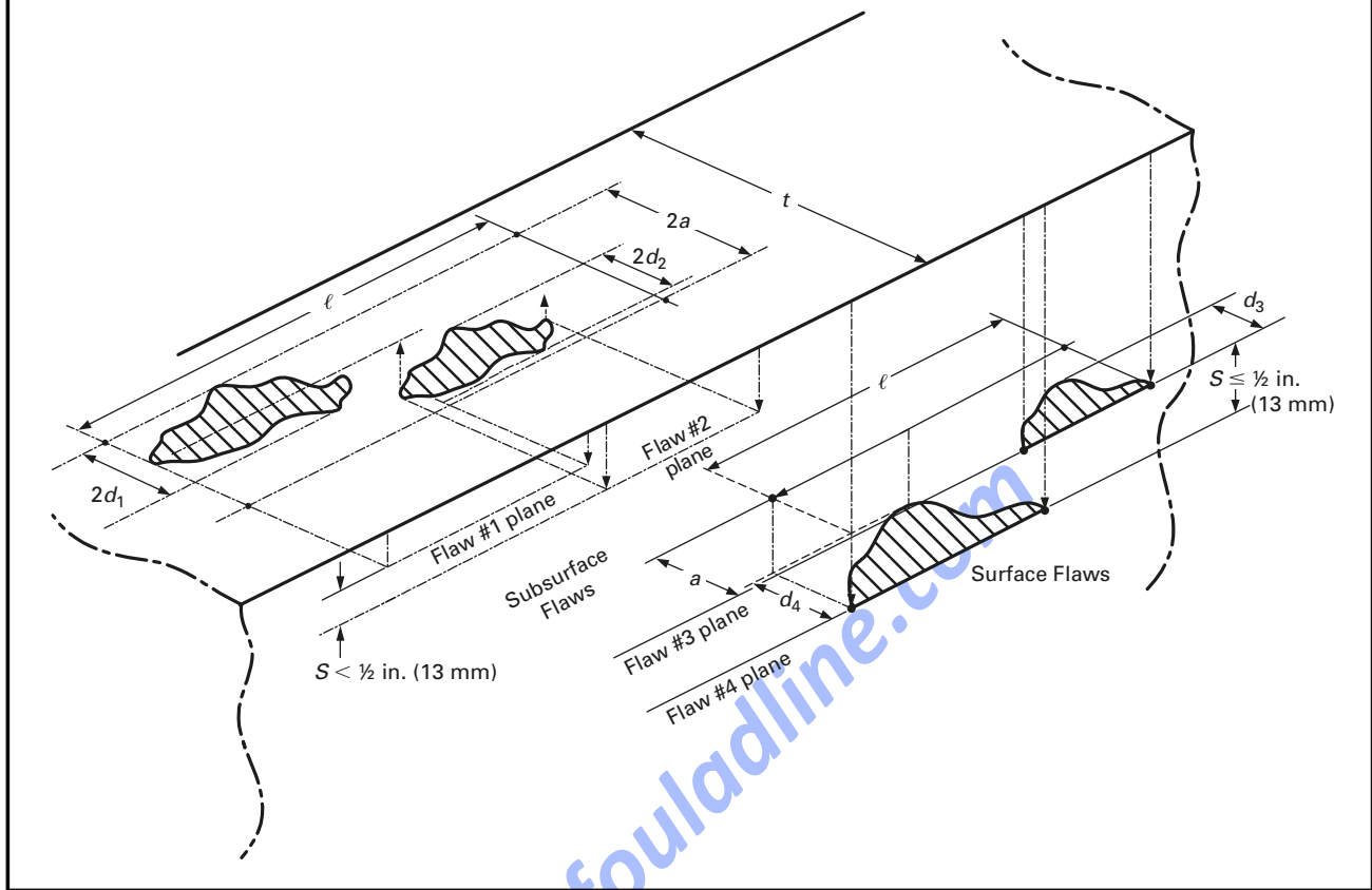
Figure 7.13 Surface and Subsurface Flaws
