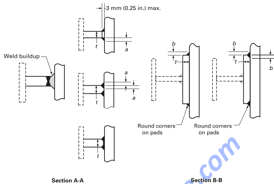
Figure 4.2.2 Some Bracket, Lug, and Stiffener Attachment Weld Details (Cont'd)
