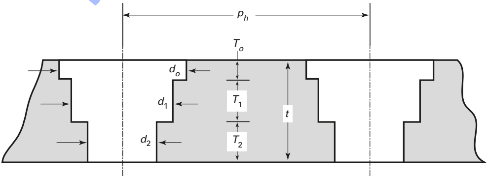
Figure 4.12.14 Multi-Diameter Holes
