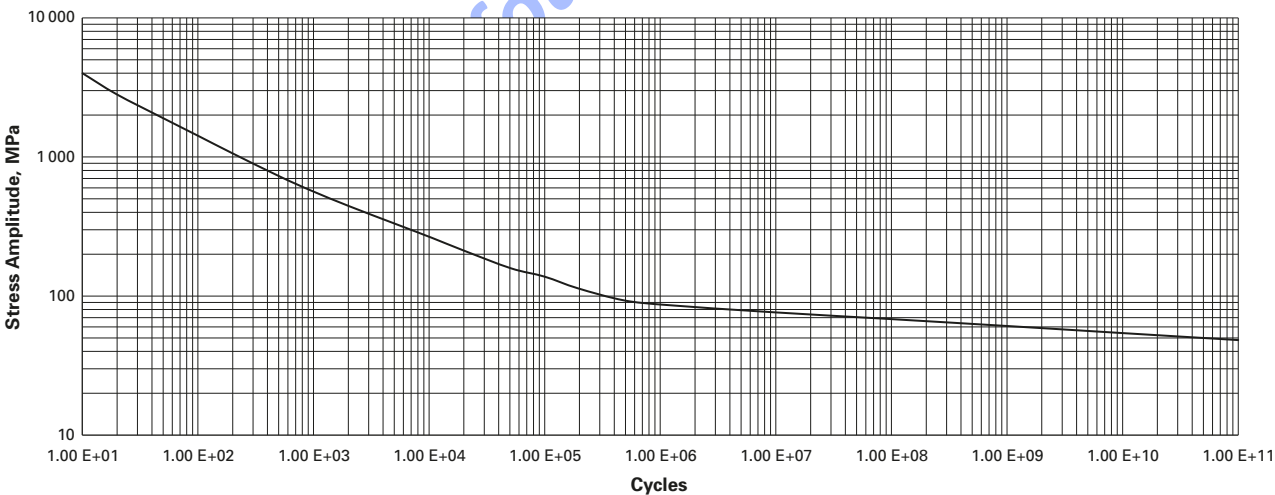
Figure 3-F.1M Fatigue Curve for Carbon, Low Alloy, Series 4XX, High Alloy, and High Tensile Strength Steels for Temperatures Not Exceeding 371°C — \sigma_{uts} \leq 552 MPa
