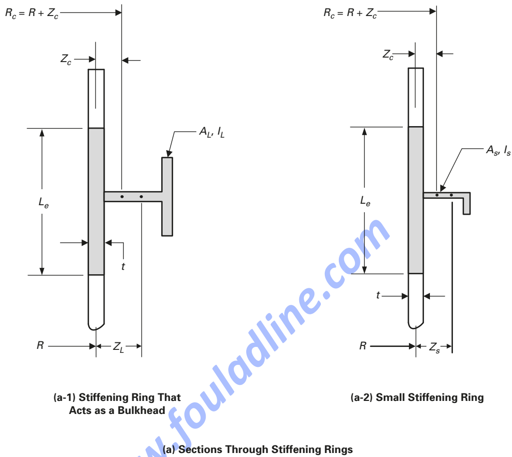
Figure 4.4.3 Stiffener Ring Parameters
