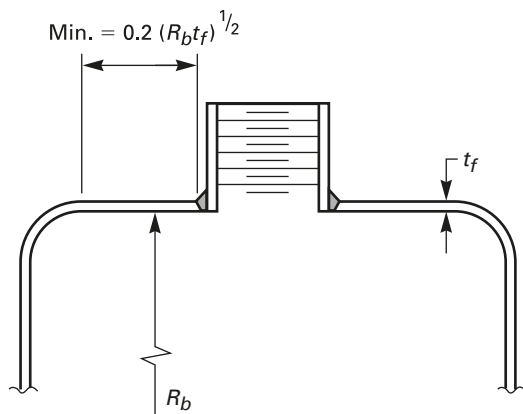
Figure 4.20.2 Typical Nozzle Attachment Details Showing Minimum Length of Straight Flange or Outer Shell Element
