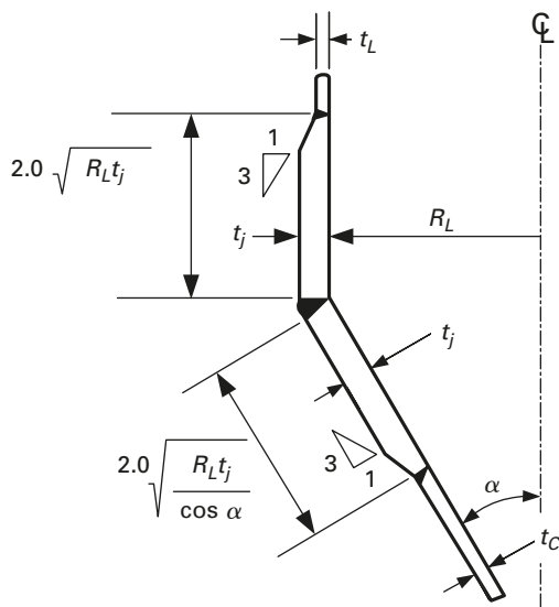
Figure 4.3.9 Reinforcement Requirements for Conical Transition Junction
