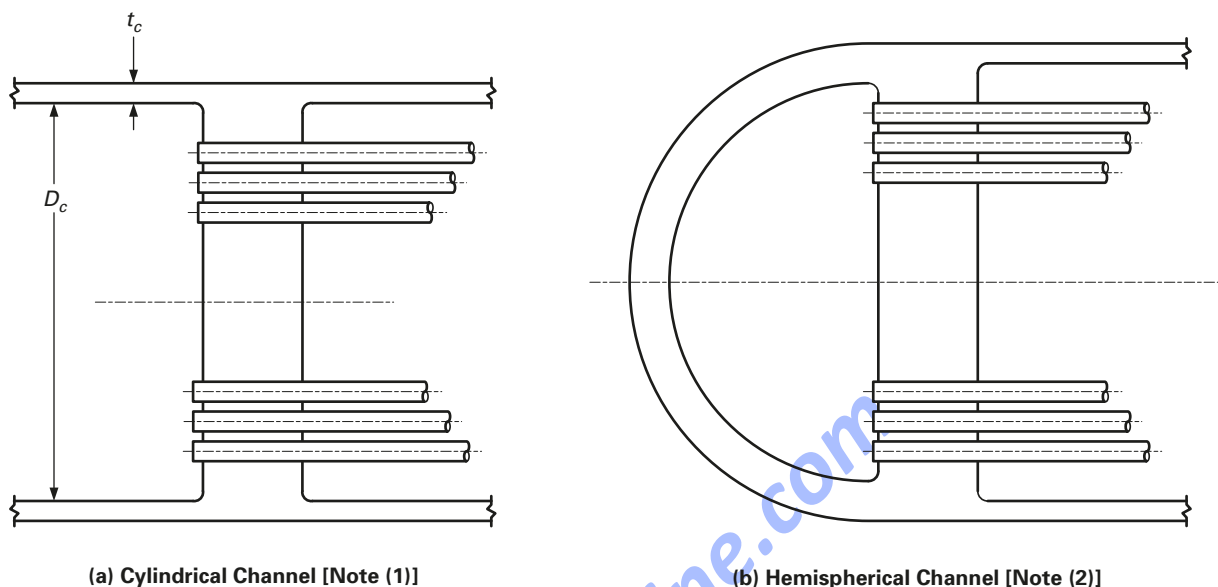
Figure 4.18.15 Integral Channels
