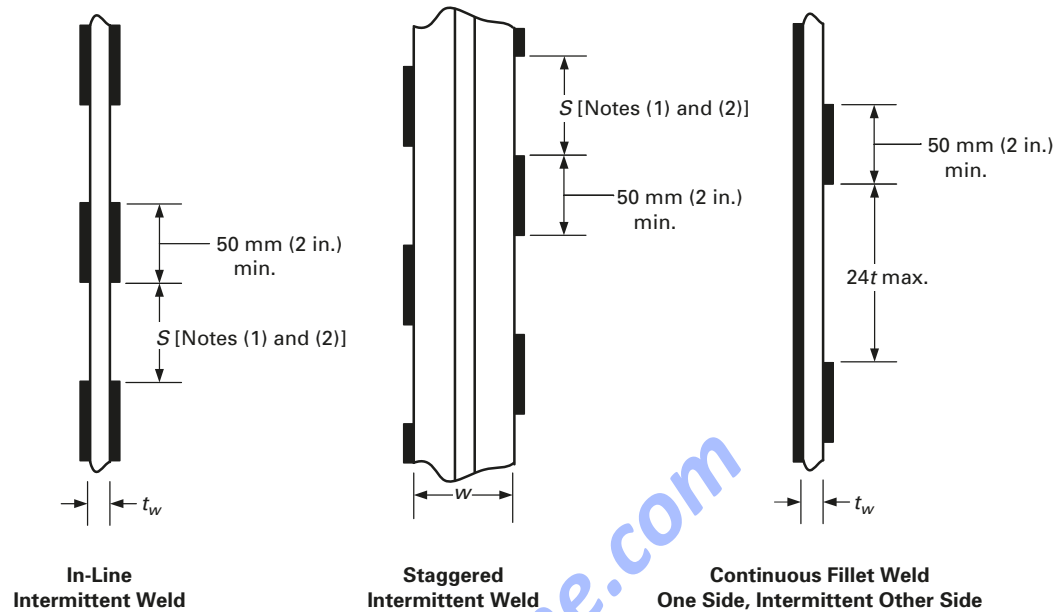
Figure 4.2.3 Some Acceptable Methods of Attaching Stiffening Rings
