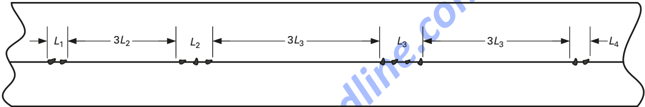
Figure 7.4 Groups of Aligned Rounded Indications
