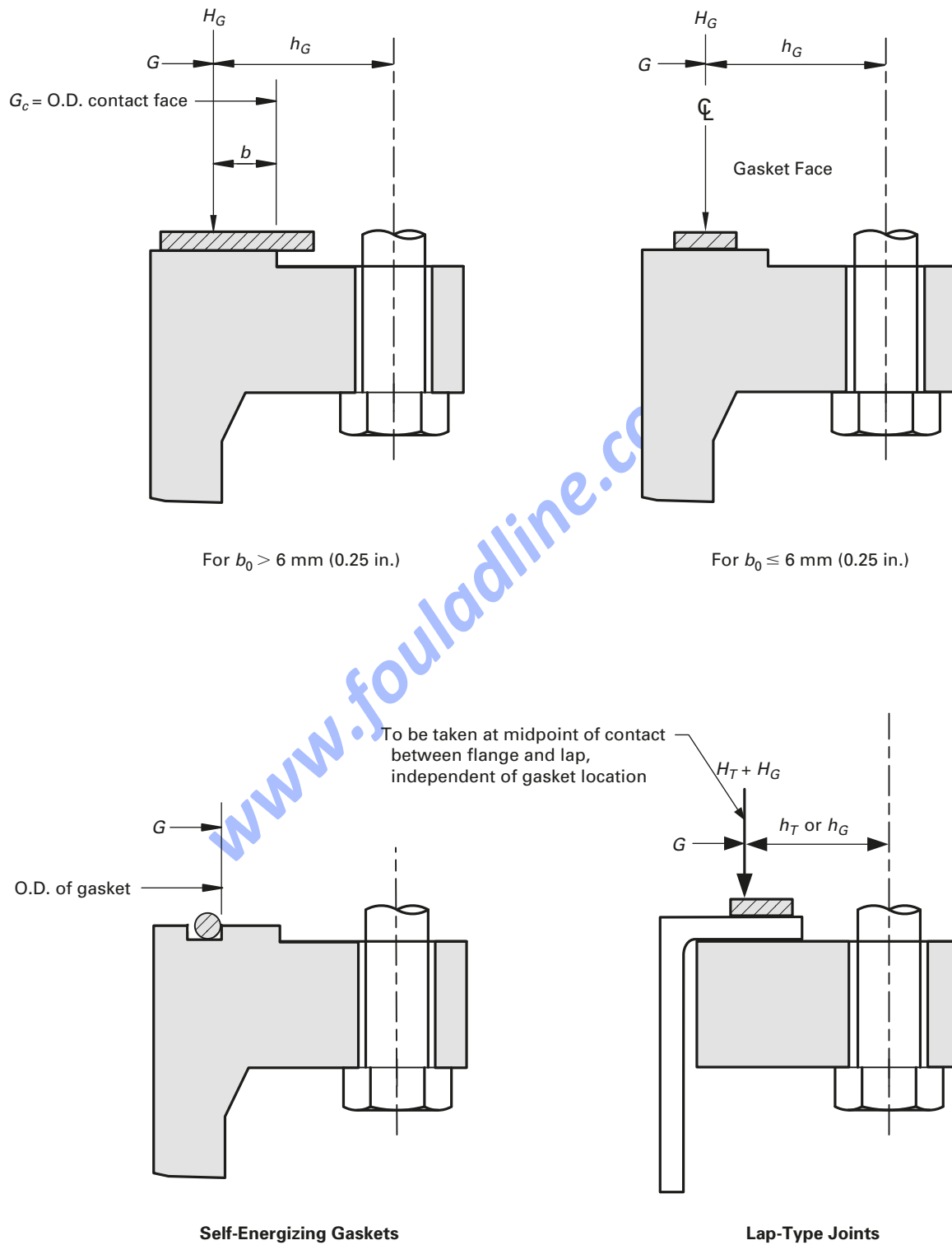
Figure 4.16.8 Location of Gasket Reaction Load Diameter
