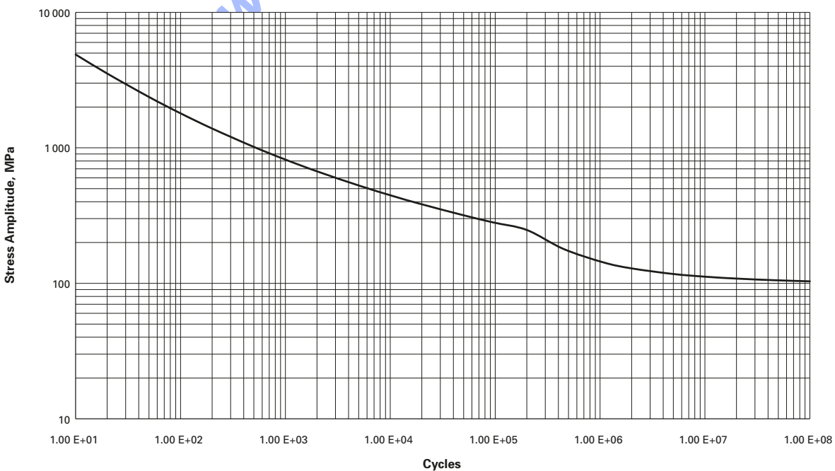
Figure 3-F.7M Fatigue Curve for Nickel–Chromium–Molybdenum–Iron, Alloys X, G, C-4, and C-276 for Temperatures Not Exceeding 427°C
