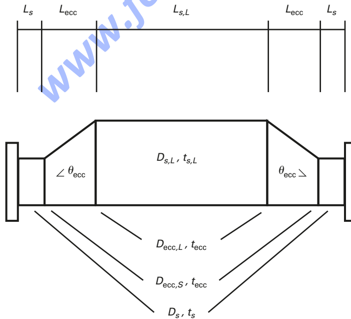
Figure 4.18.17 Kettle Shell
