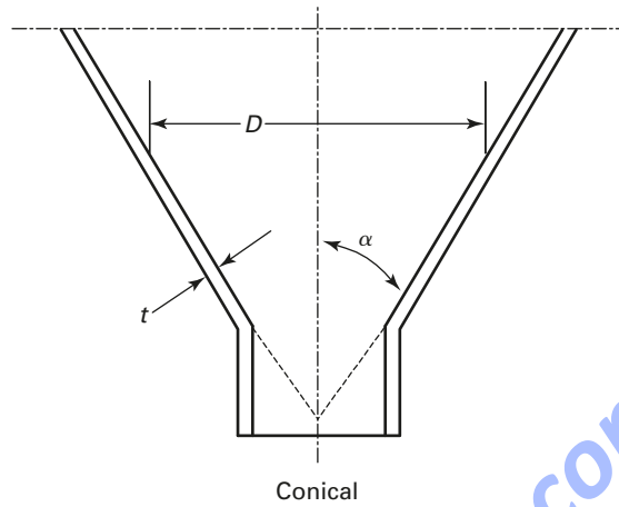
Figure 4.3.1 Conical Shell
