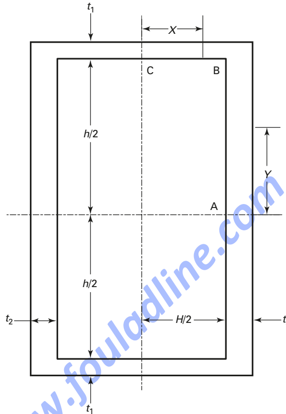
Figure 4.12.1 Type 1 Noncircular Vessels (Rectangular Cross Section)
