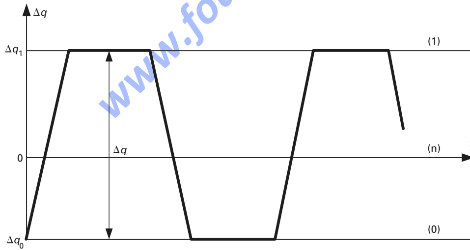
Figure 4.19.9 Cyclic Displacements
