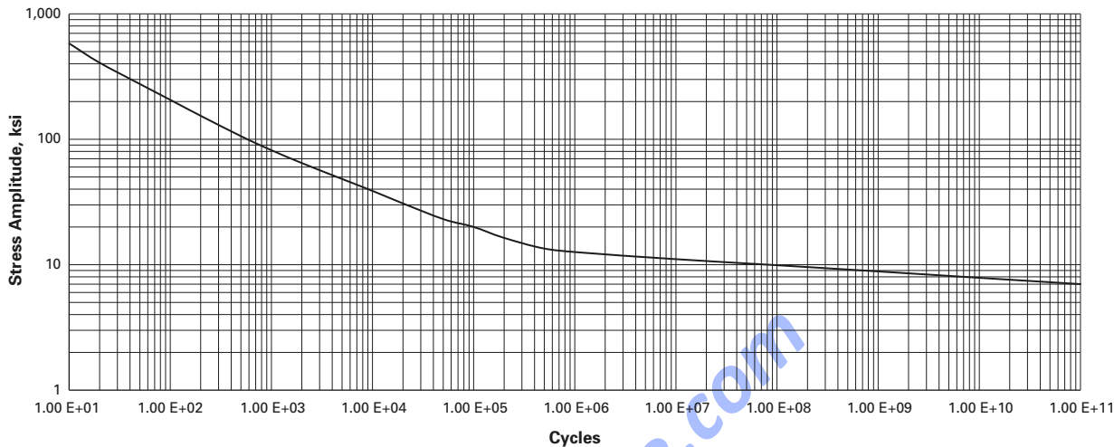
Figure 3-F.1 Fatigue Curve for Carbon, Low Alloy, Series 4XX, High Alloy, and High Tensile Strength Steels for Temperatures Not Exceeding 700°F — \sigma_{uts} \leq 80 ksi
