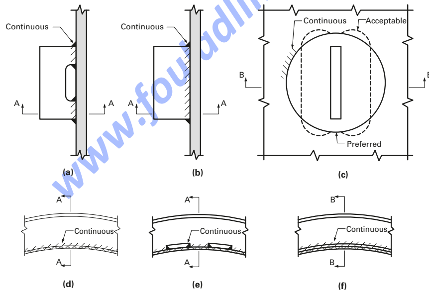
Figure 4.2.2 Some Bracket, Lug, and Stiffener Attachment Weld Details
