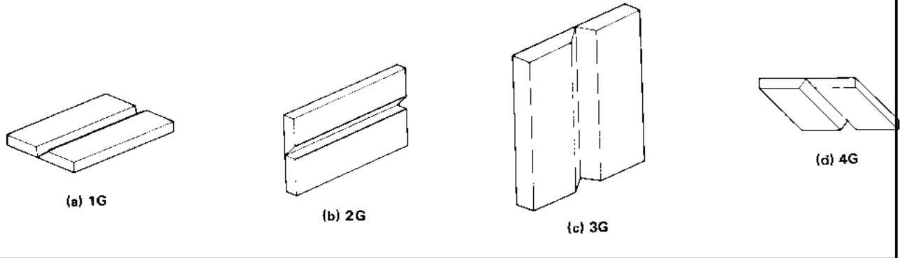
Figure QW-461.3 Groove Welds in Plate — Test Positions
