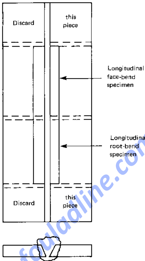
Figure QW-463.2(c) Plates — Longitudinal Performance Qualification
